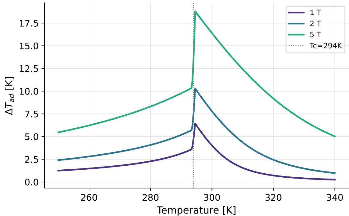
Adiabatic Temperature Change
