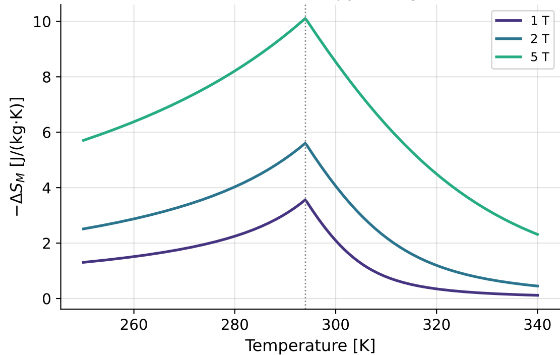
Isothermal Entropy Change
