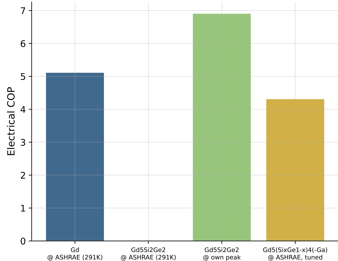
Electrical COP
