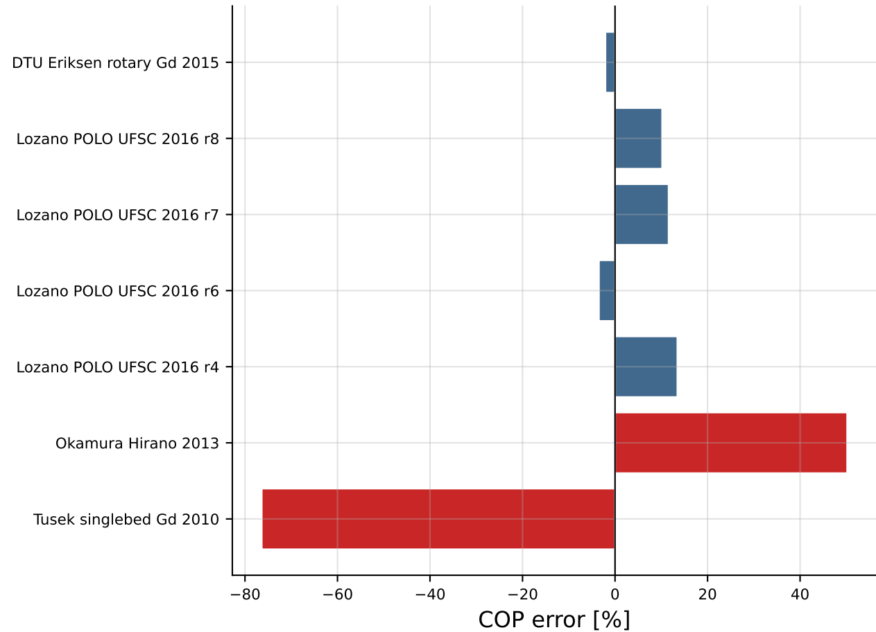
COP Prediction Error by Device
