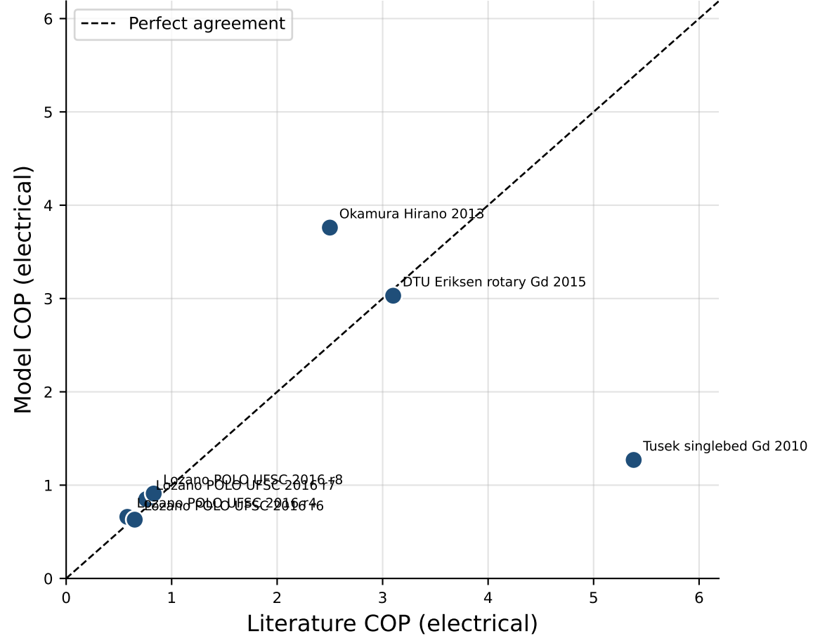
System-Level Validation: Model vs. Literature (fluid m \dot{m} calibrated to reproduce reported Q _c )
