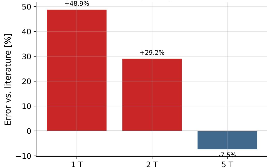
Model Error (mean-field theory overpredicts near T_c )
