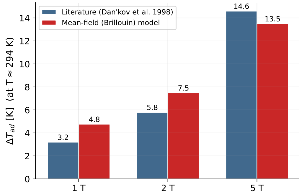
Gd Adiabatic Temperature Change: Model vs. Literature
