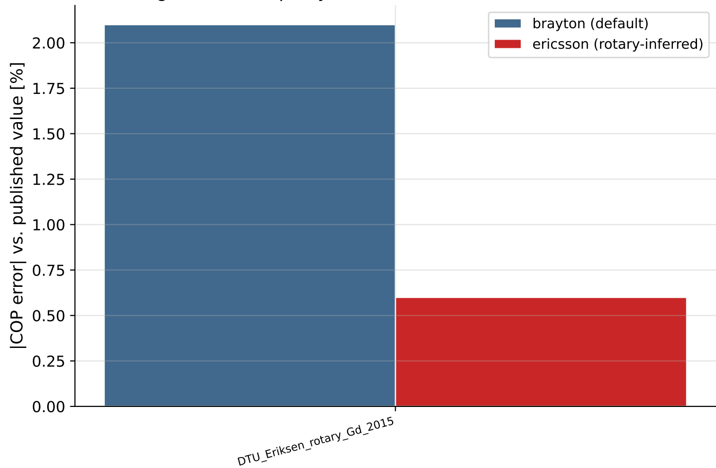
Cycle-Topology Sensitivity: Rotary Benchmark Devices (naming-convention proxy, not a literature-confirmed classification)
