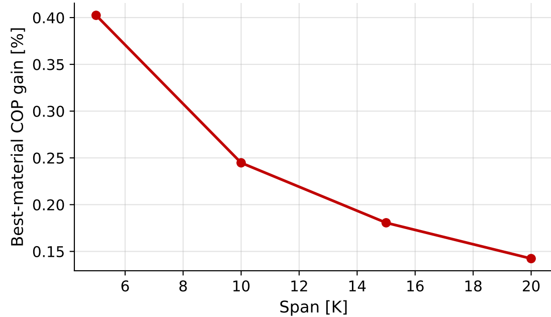
Gain vs. Span (alignment window widens/narrows with span)
