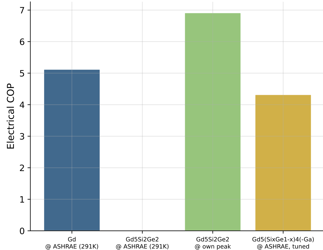
Electrical COP
