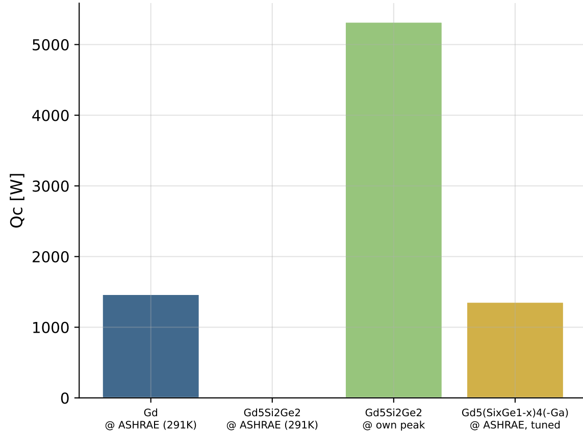
Cooling Capacity
