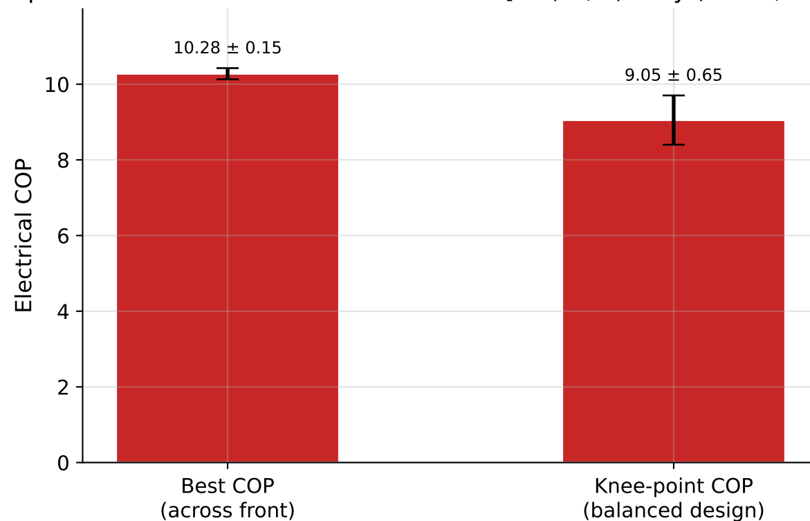
Headline COP Numbers, Mean \pm Std Knee-point material consistent across seeds: ['La(Fe,Si) 13 Hy (tuned, T c =285.3K)']
