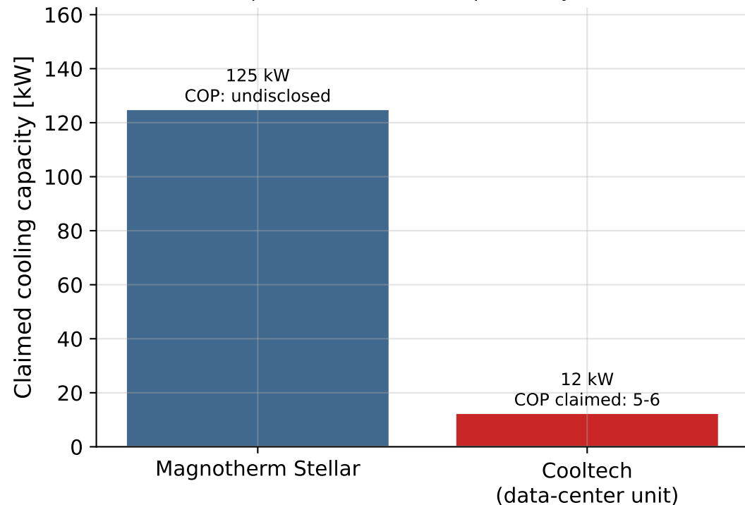
Commercial Magnetocaloric-AMR Claims (trade-press/vendor, not independently audited)
