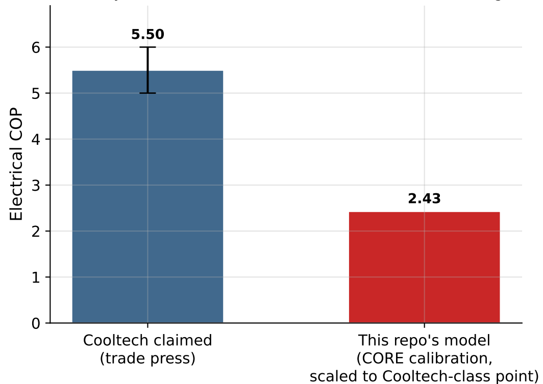
Model vs. Cooltech's Own Claim gap vs. claimed midpoint: -56% (already-documented calibration limitation, not a new finding)
