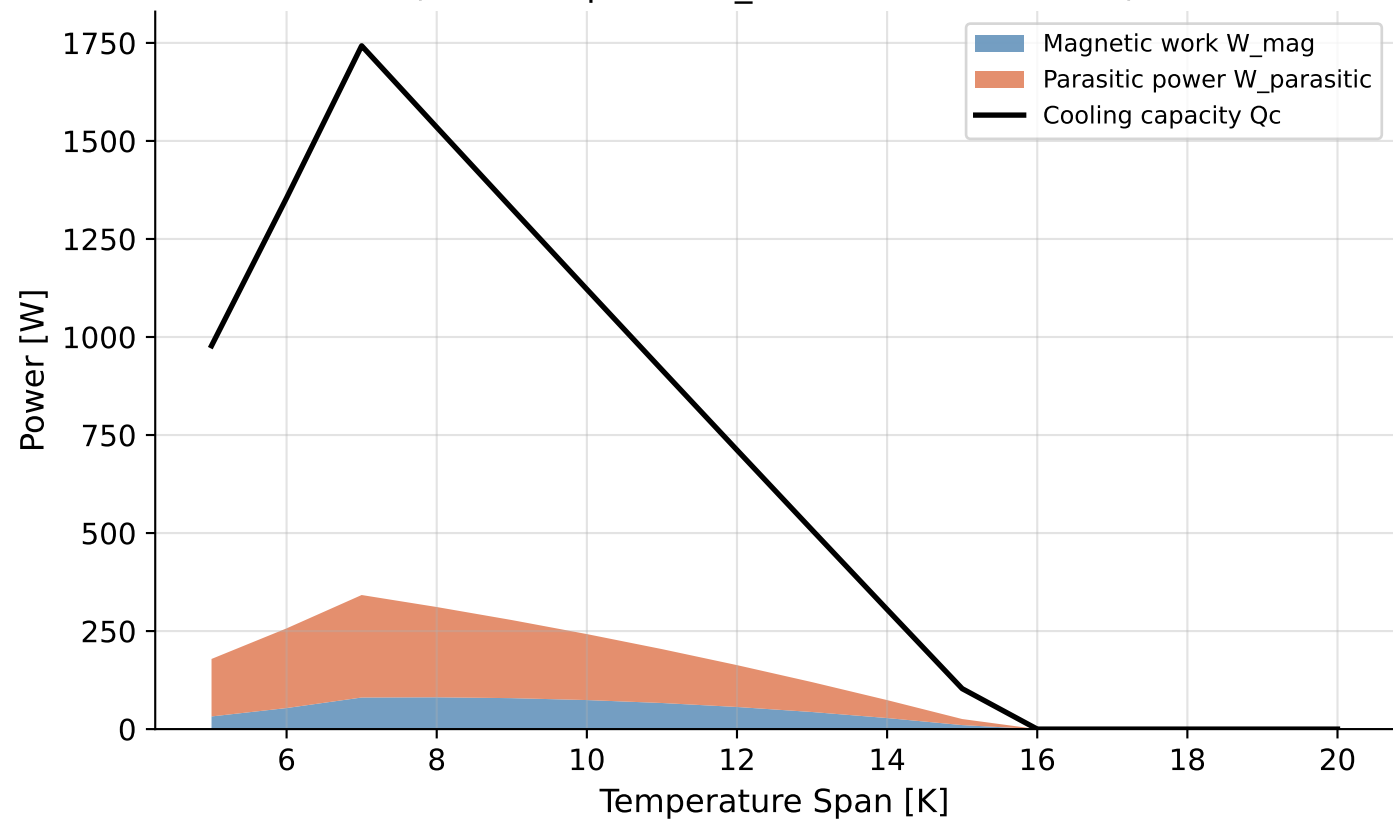
AMR Energy Balance vs. Span (constant parasitic_fraction=0.15 default)
