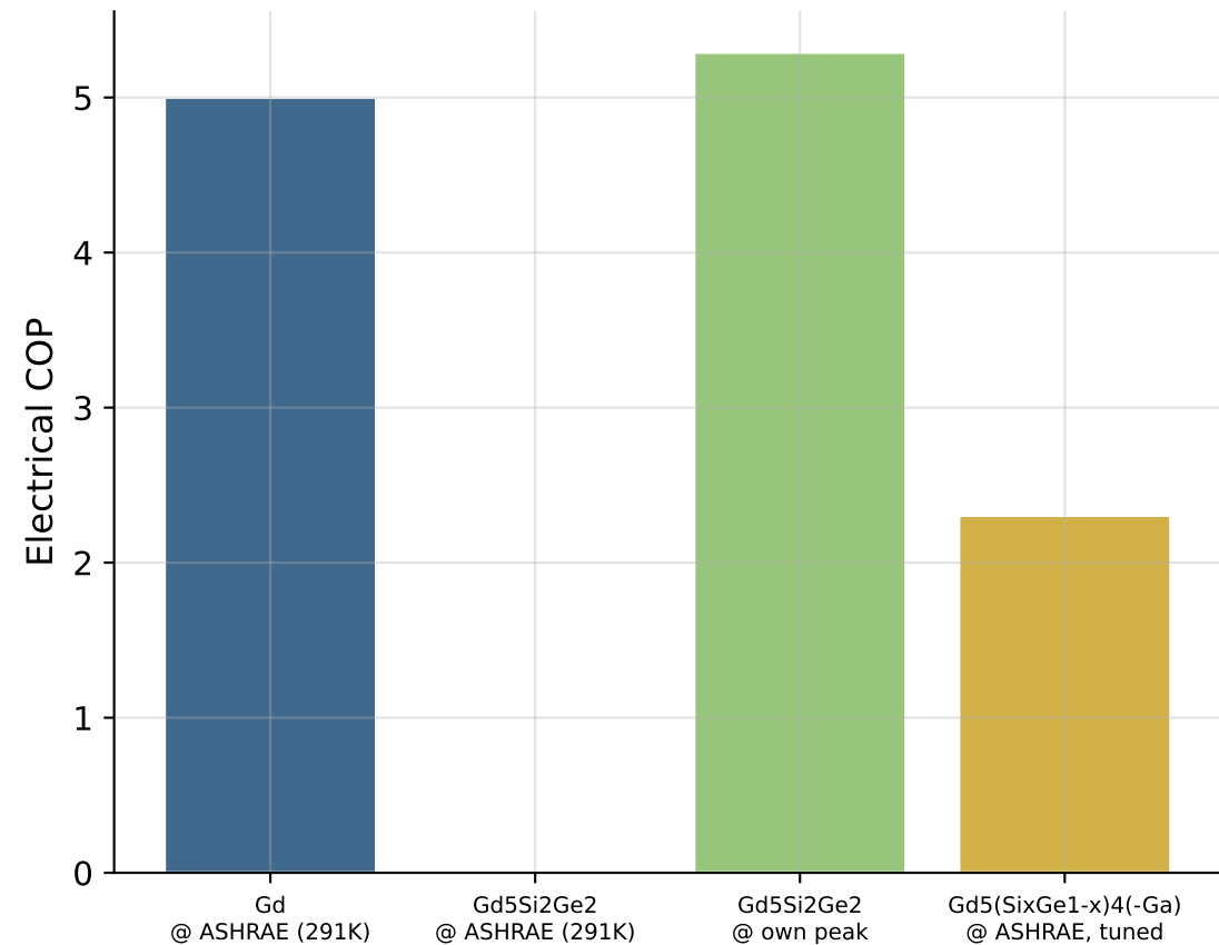
Electrical COP
