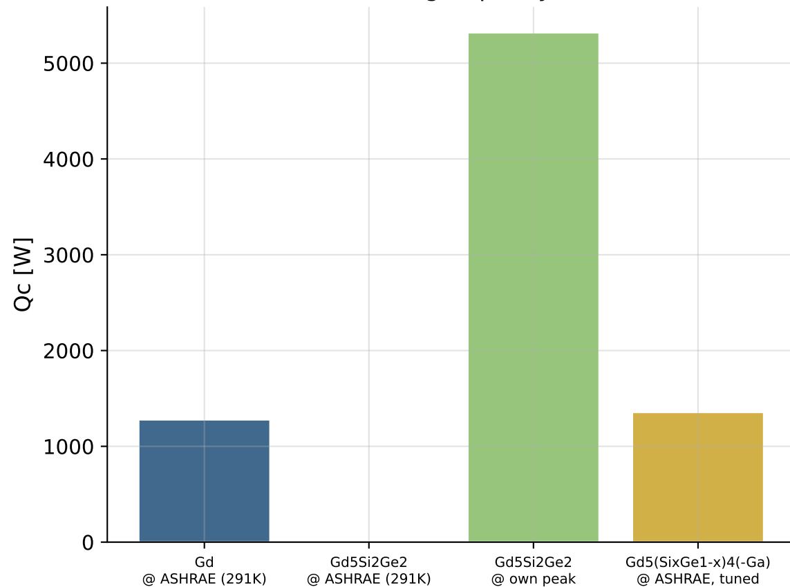
Cooling Capacity
