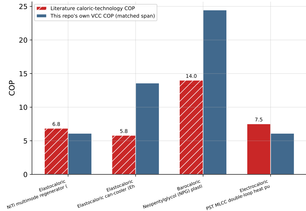
Literature Claims vs. This Repo's VCC (hatched = simulation/projection/vendor claim, not a measured device)
