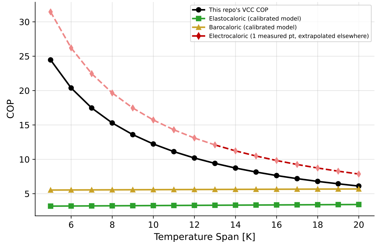
Physics-Model Span Sweep (this repo's own literature-calibrated models, same grid as comparison_table.csv)
