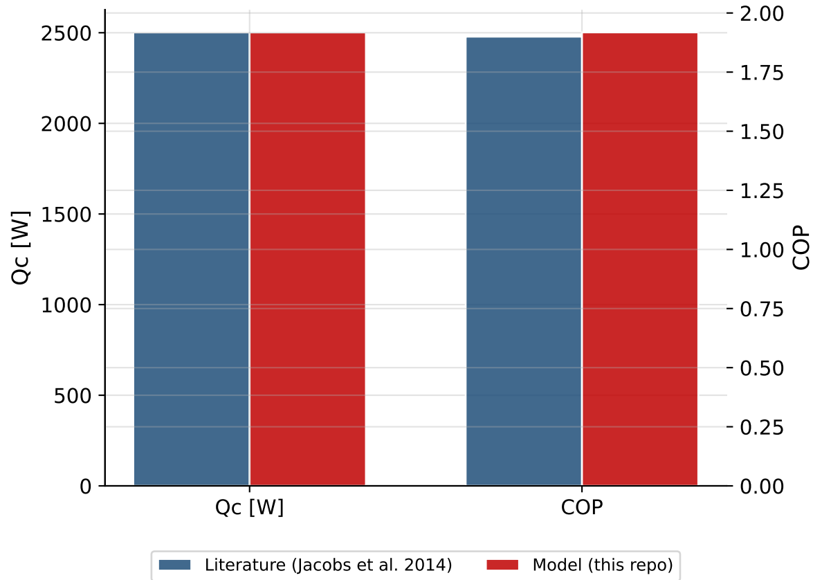
Astronautics_rotary_2014 Validation COP error: +0.9%
