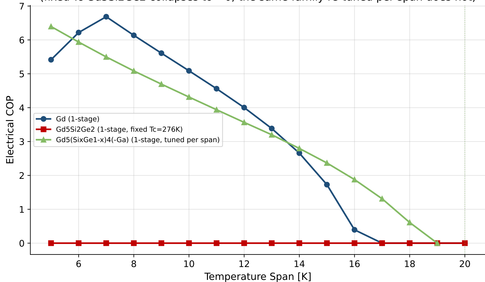
Gd vs. Gd 5 Si 2 Ge 2 in the ASHRAE Range (fixed-T c Gd 5 Si 2 Ge 2 collapses to ~0; the same family re-tuned per span does not)
