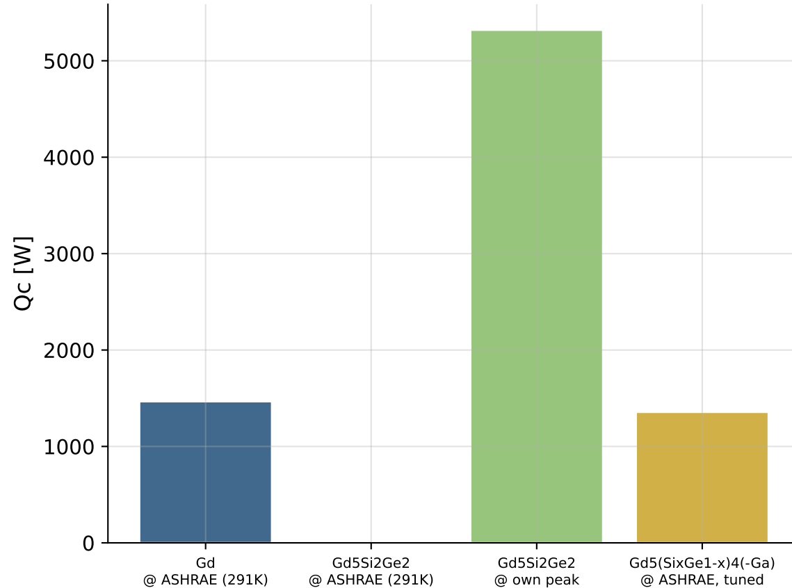
Cooling Capacity
