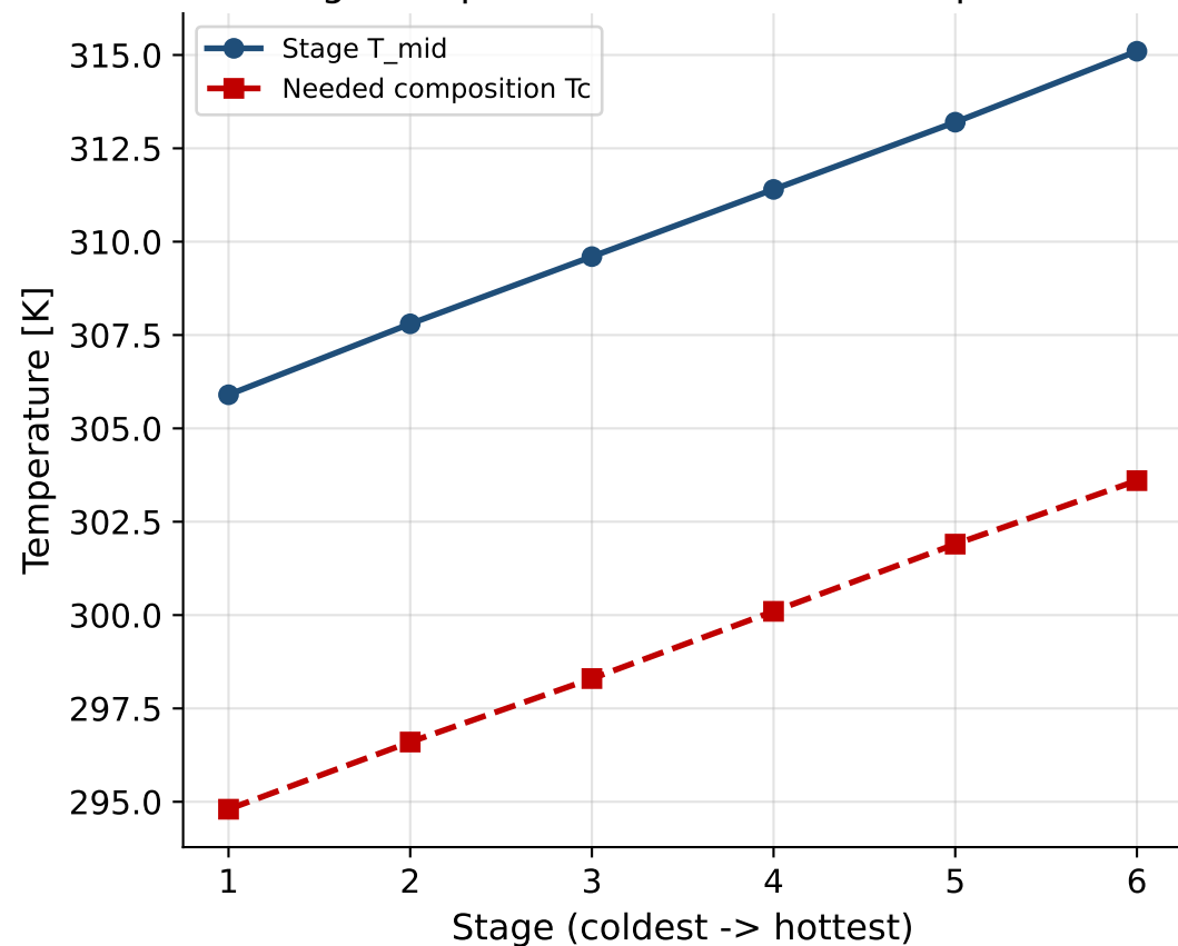
6-Layer Curie-Graded Bed: Stage Temperature vs. Needed Composition
