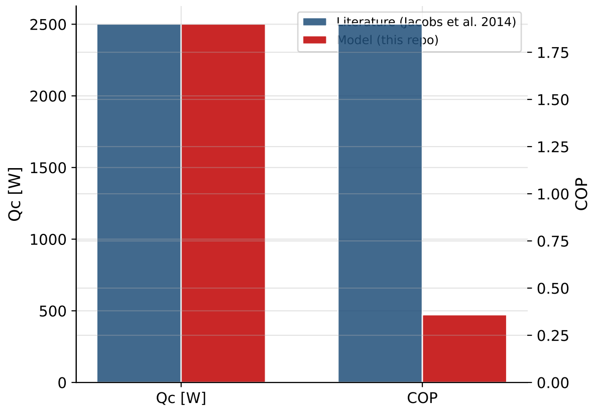
Astronautics_rotary_2014 Validation COP error: -81.1%
