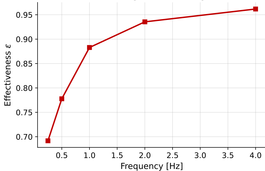
\varepsilon vs. Frequency (mass=2kg, \dot{m}=0.08\text{kg/s} )
