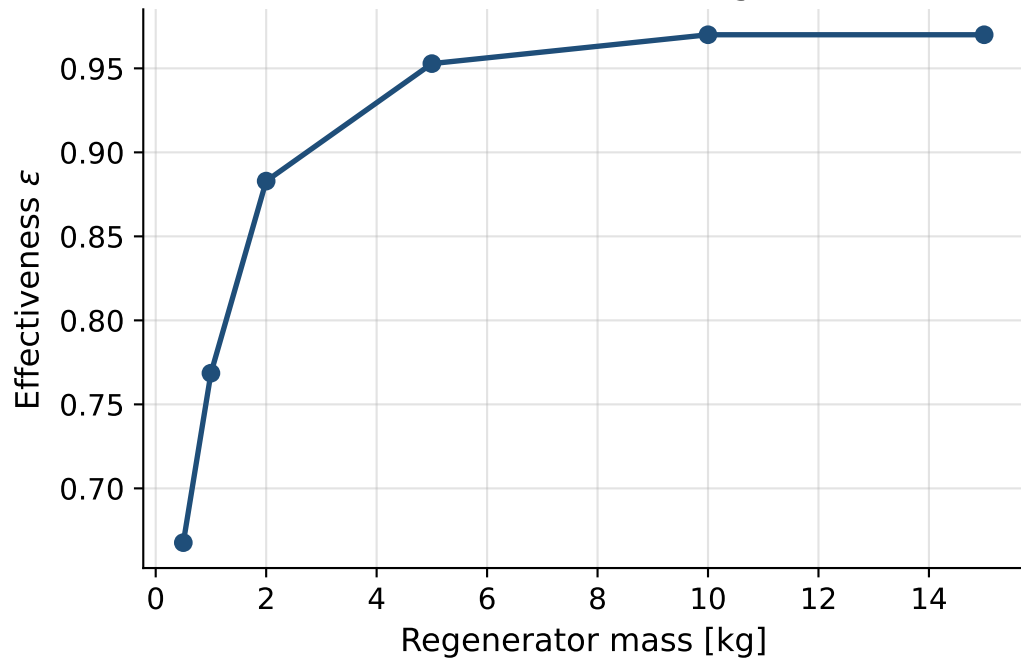
\varepsilon vs. Regenerator Mass ( f=1\text{Hz} , \dot{m}=0.08\text{kg/s} )
