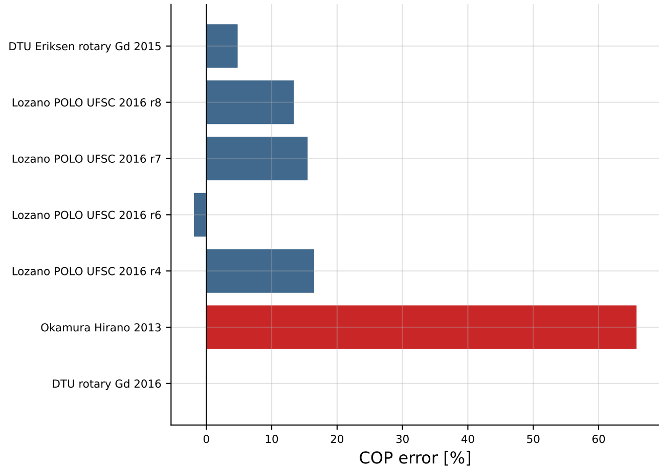
COP Prediction Error by Device
