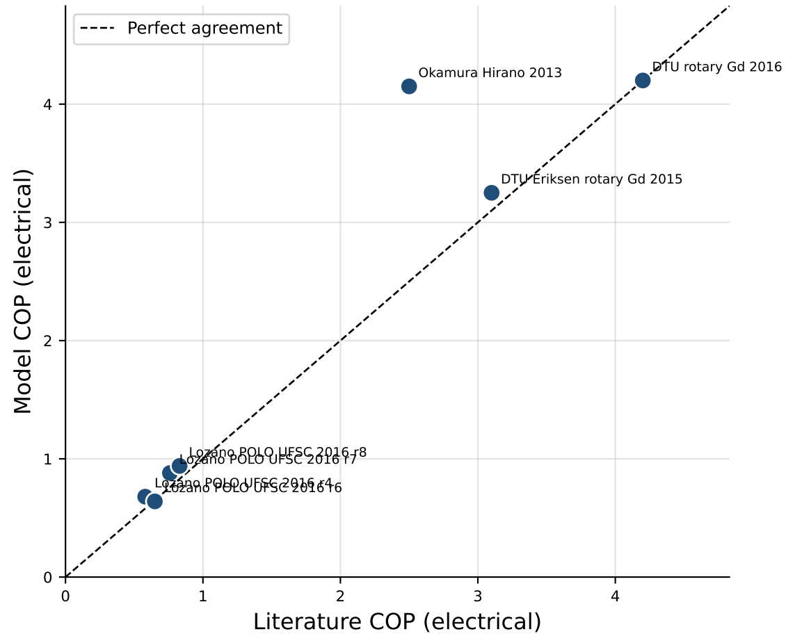
System-Level Validation: Model vs. Literature (fluid mdot calibrated to reproduce reported Qc)
