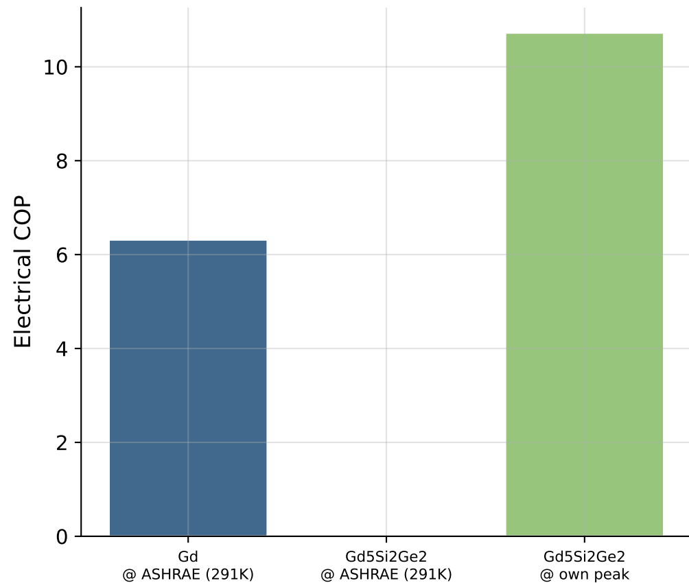
Electrical COP
