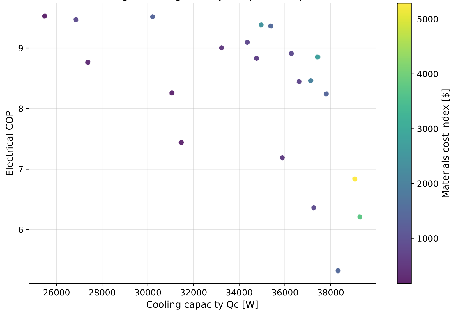
NSGA-III Pareto-Optimal AMR Designs ( T_{\text{cold}}=291\text{K} , span=10K; state-dependent loss + NTU thermal model; material + regenerator geometry co-optimized, phase 15)
