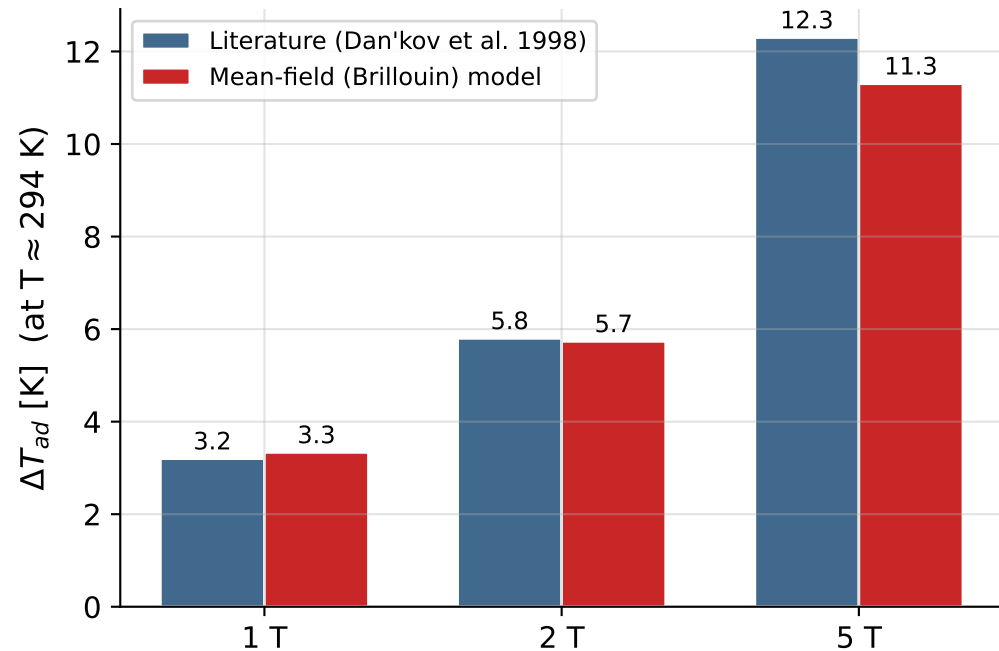
Gd Adiabatic Temperature Change: Model vs. Literature
