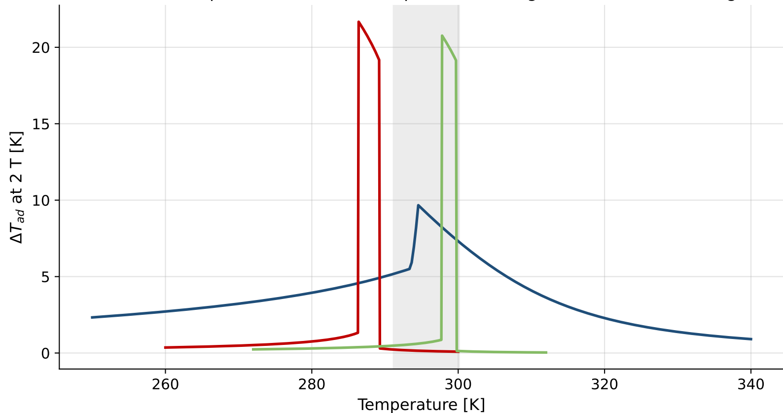
Material Comparison: Adiabatic Temperature Change vs. Data-Center Range
