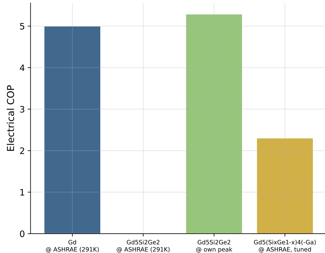
Electrical COP
