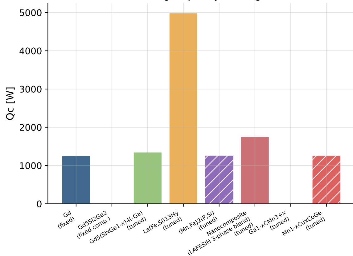
Cooling Capacity (1-stage)
