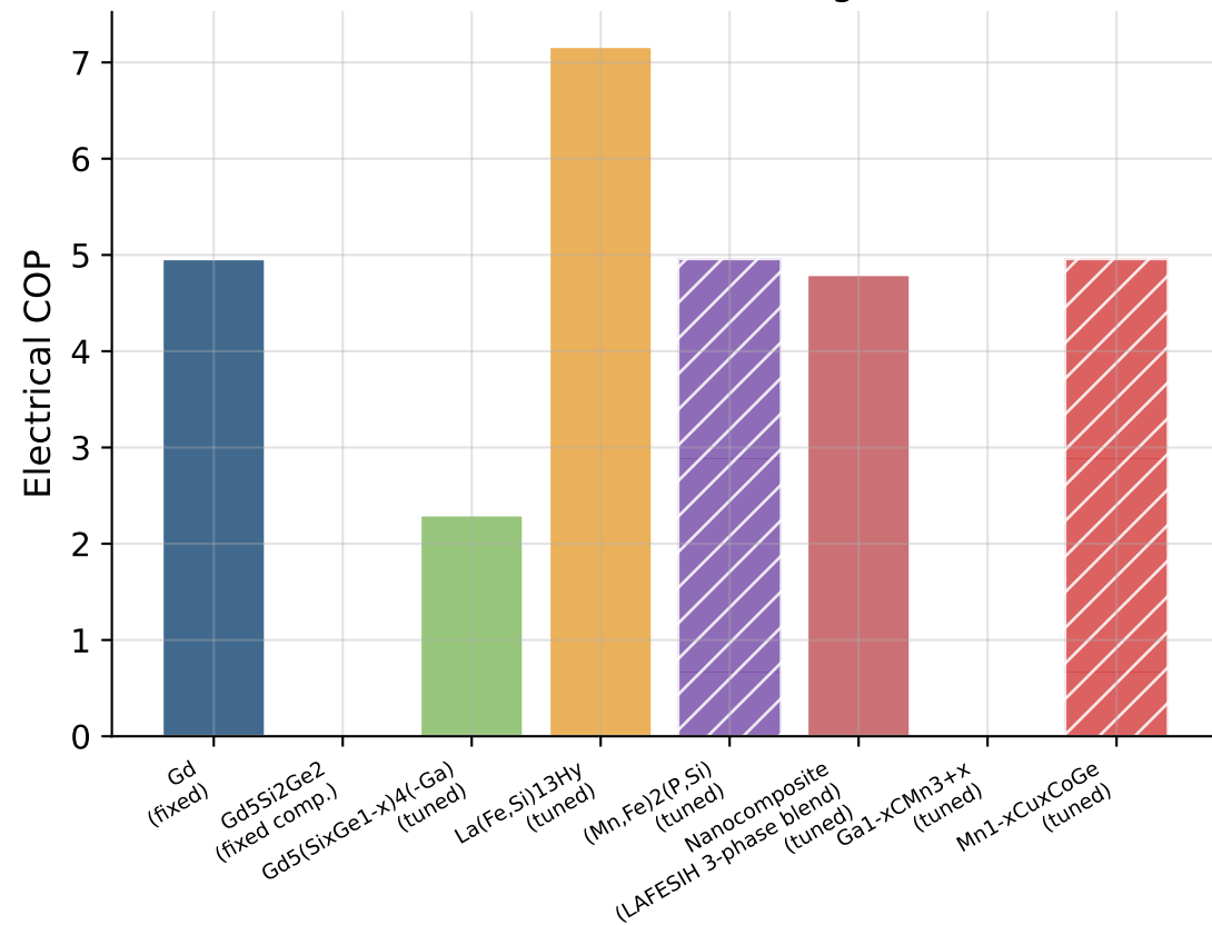
Electrical COP (1-stage)
