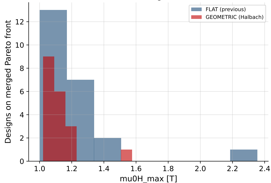
Field-Strength Distribution FLAT vs. GEOMETRIC magnet-mass cost term
