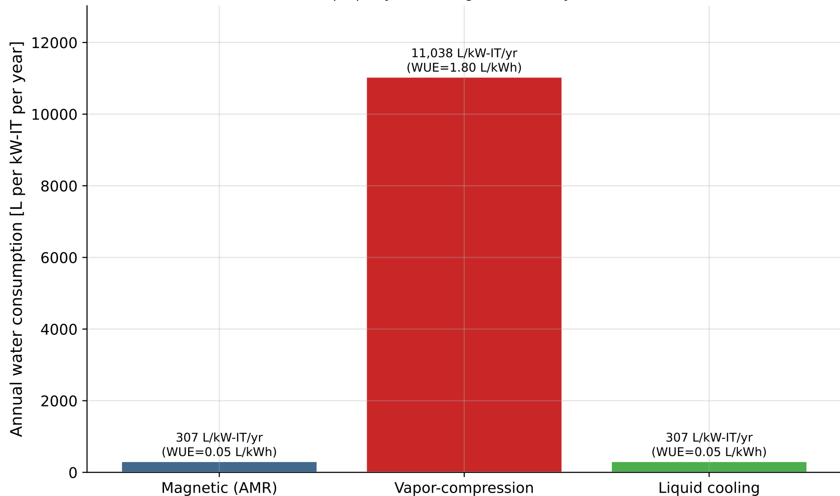
Annual Water Usage (WUE) Comparison, 100kW-IT Facility (AMR assigned dry/air-cooled rejection by default — a design choice, not a property of the magnetocaloric cycle itself)
