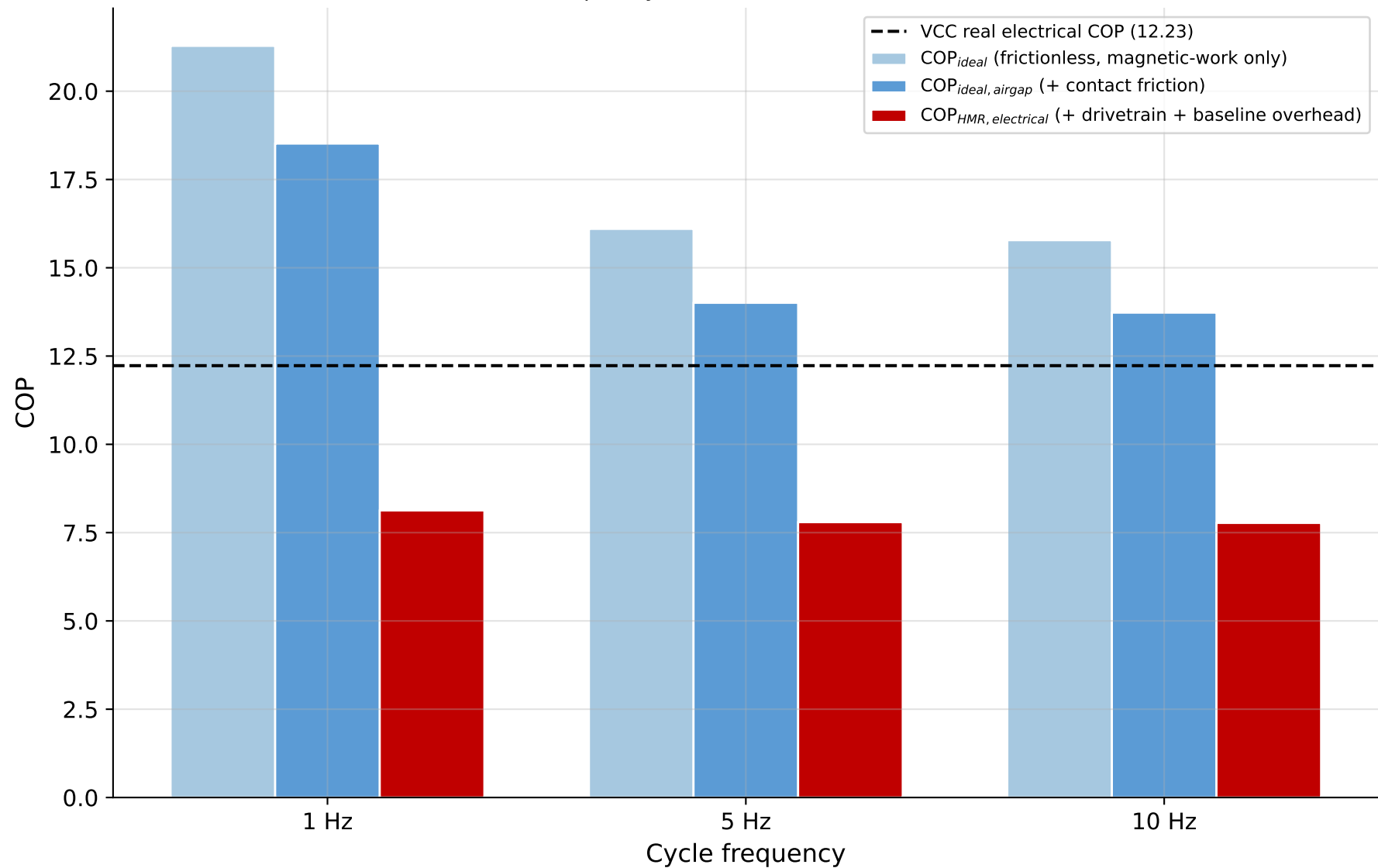
Hybrid Solid-State Regenerator (HMR) vs. VCC: Ideal \rightarrow Real (Lin et al. 2024, Gd/Cu; best-frequency HMR real electrical COP does NOT beat VCC's, 0.66\times )
