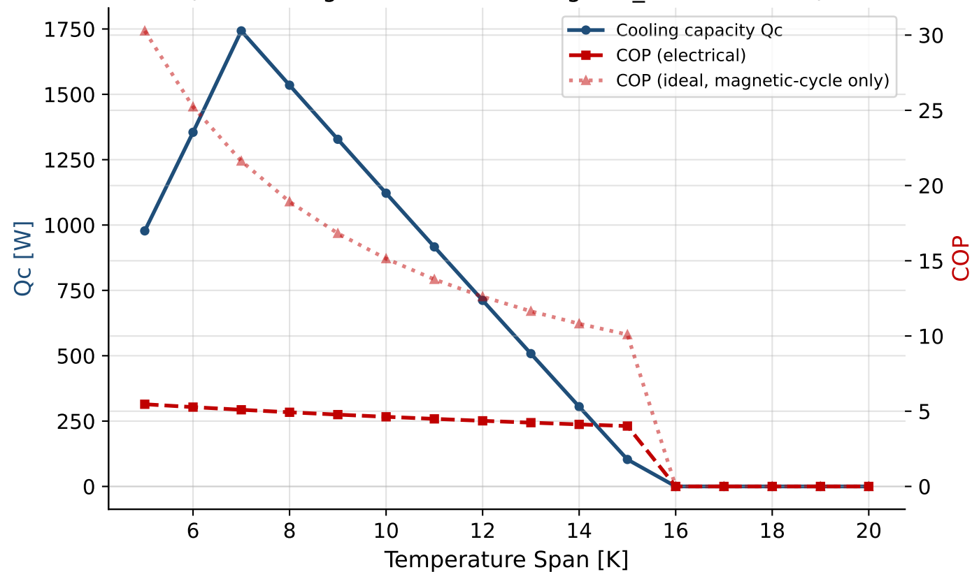
Single-Stage AMR Characteristic Curve (Gd, 2T, 5kg, 2Hz, \dot{m}=0.08\text{kg/s} , T_{\text{cold}}=291.15\text{K} )
