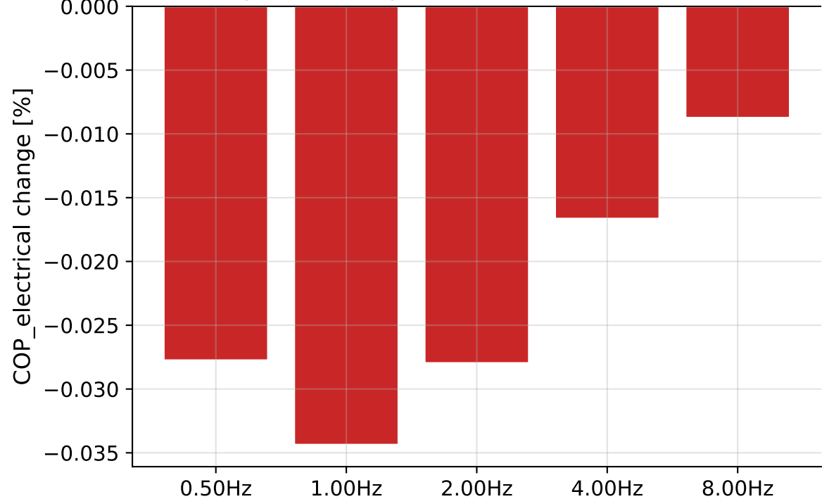
Diode Actuation-Cost Penalty (cost-only accounting, no rectification benefit modeled)
