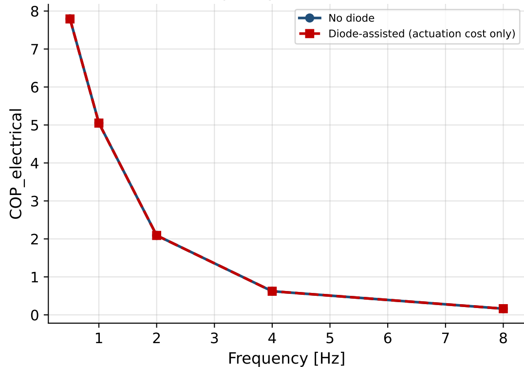
COP vs. Frequency, With/Without Diode
