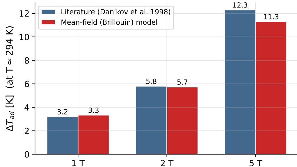
Gd Adiabatic Temperature Change: Model vs. Literature
