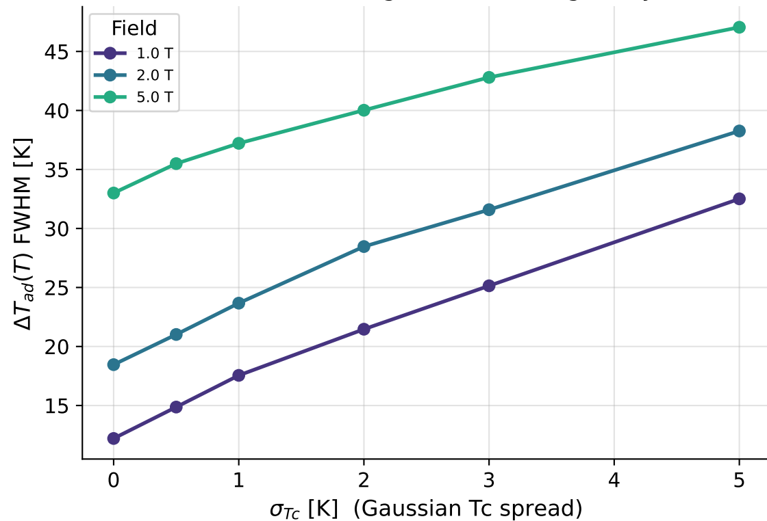
Peak Broadening vs. Tc Inhomogeneity
