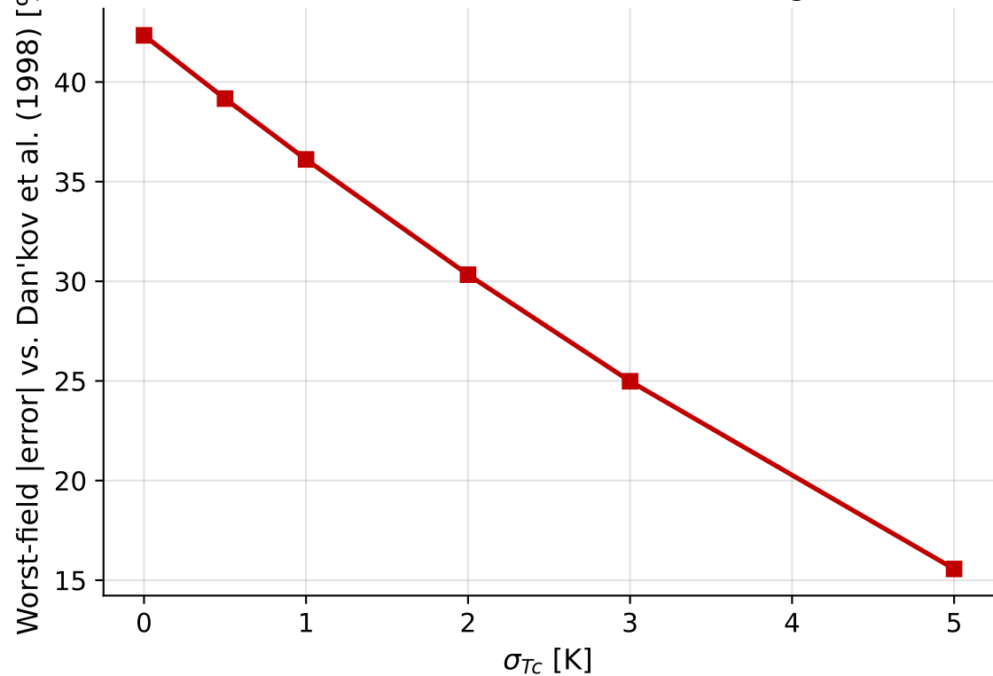
Validation Error vs. Tc-Broadening
