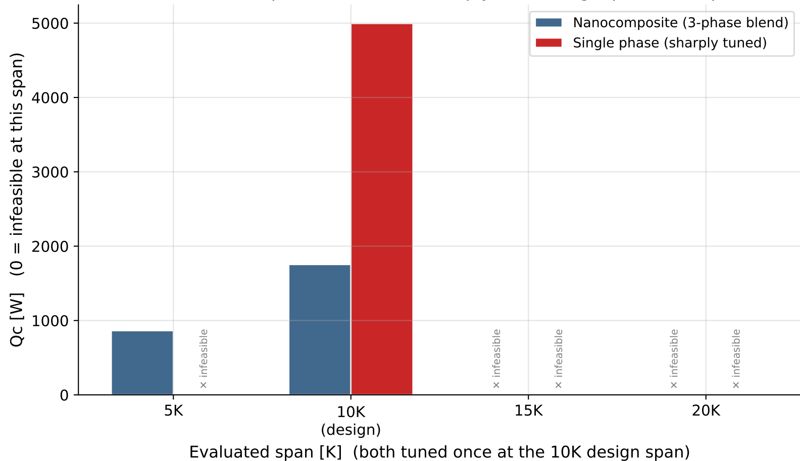
Nanocomposite Off-Design Robustness Broad blend keeps Q_c > 0 where a sharply-tuned single phase collapses
