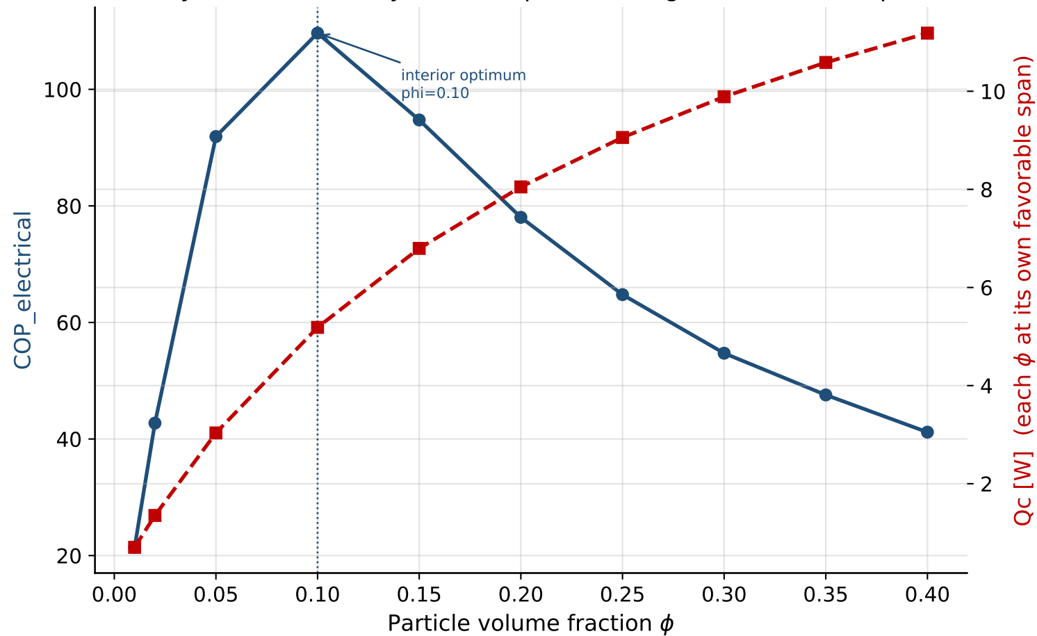
Ferrofluid/MR-Suspension MCE — Volume-Fraction Trade-off Viscosity-vs-MCE-intensity trade-off produces a genuine interior optimum
