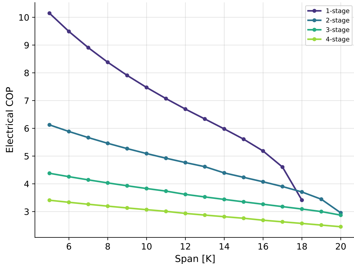
Curie-Graded Cascade COP
