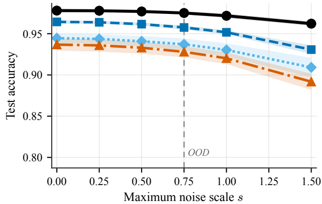
Fashion-MNIST -- heterogeneous Gaussian noise
