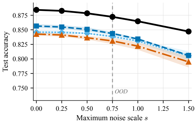
Fashion-MNIST -- heterogeneous Gaussian noise
