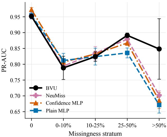
APS -- predictive performance by missingness
