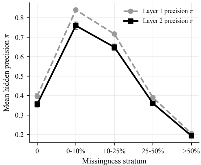
BVU -- internal precision by missingness
