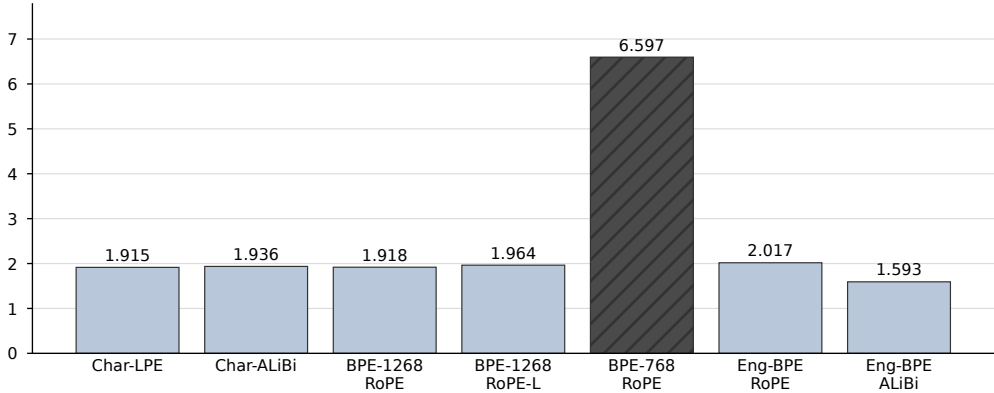
Held-out BPB
