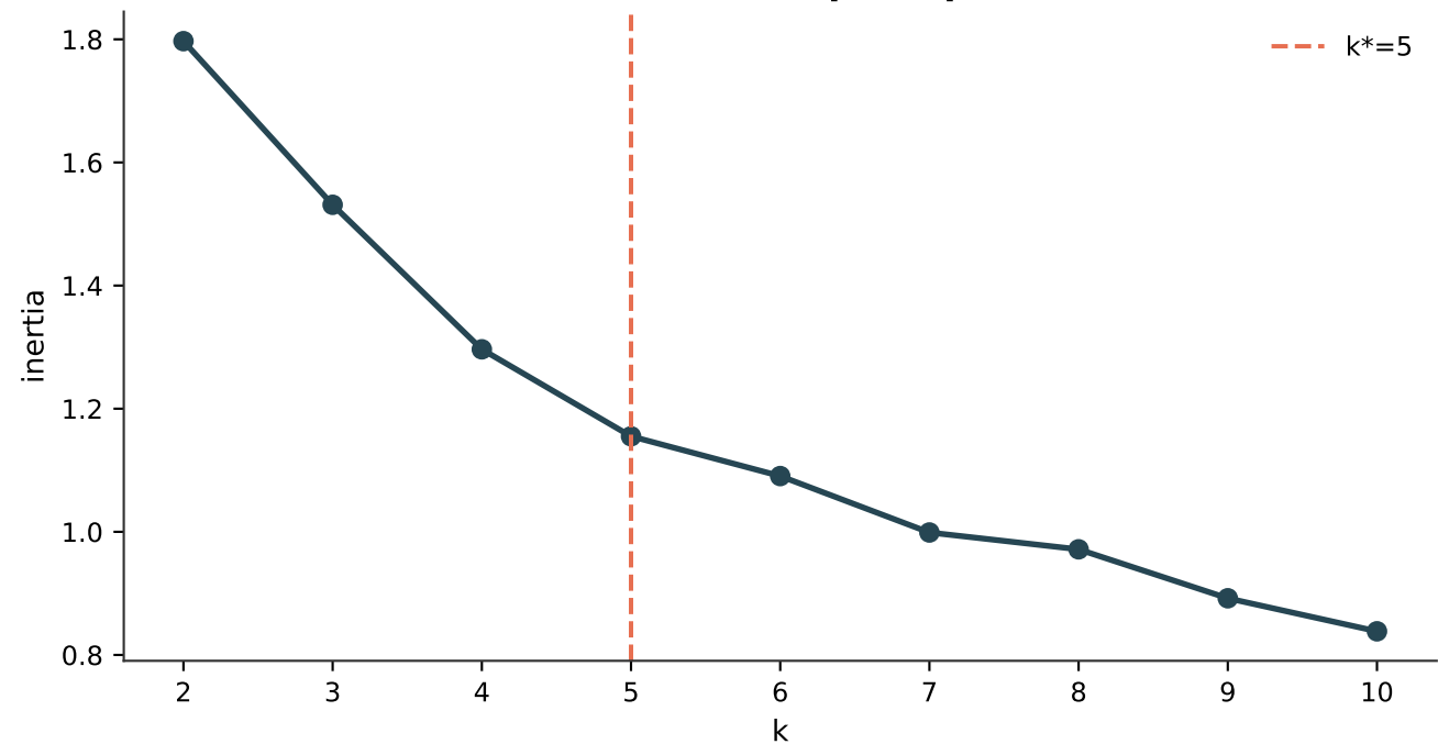
K-means elbow — consumption profile clusters
