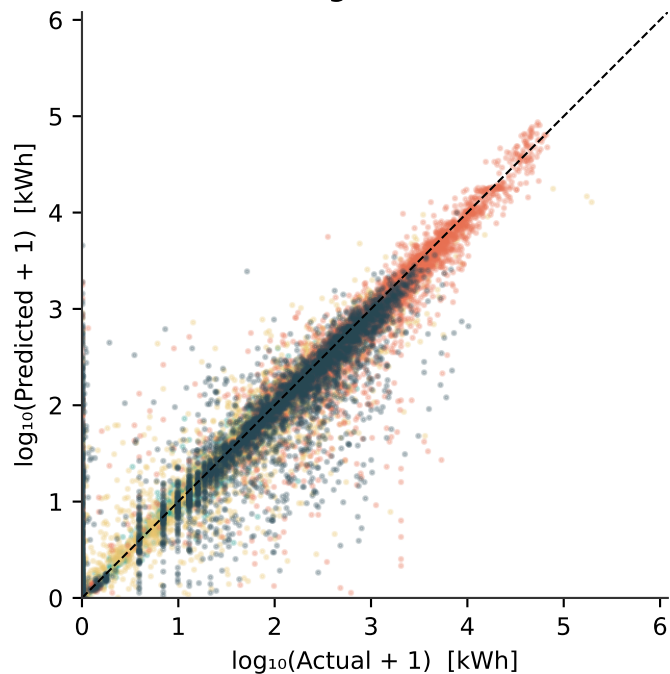
LightGBM
