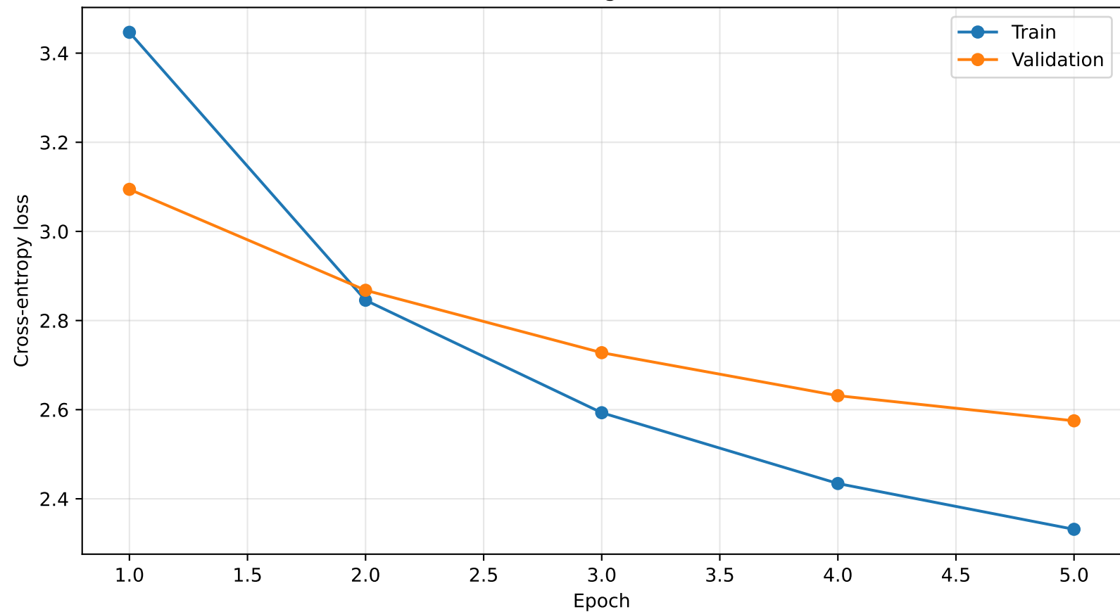
Training Loss
