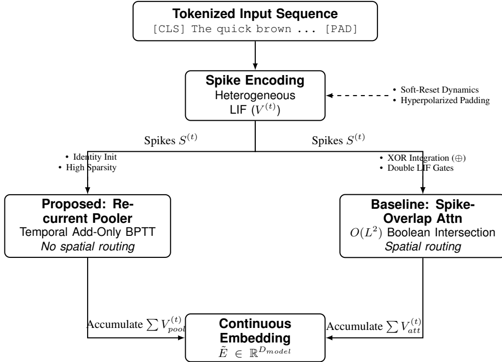
Figure 1: Architectural flowchart contrasting the proposed minimalist Recurrent Pooler against the \mathcal{O}(L^2) Spike-Overlap Attention baseline. The Recurrent Pooler completely bypasses quadratic spatial routing, natively translating discrete token spikes into a continuous temporal embedding state.
