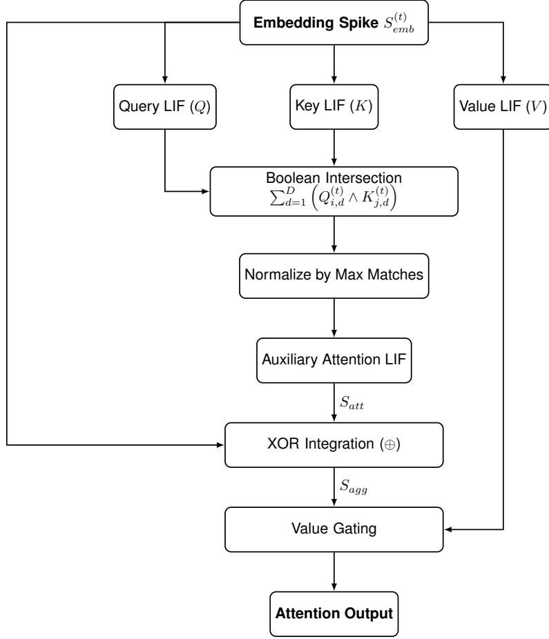
Figure 2: Detailed computational flow of the Spike-Overlap Attention mechanism at a single timestep.
