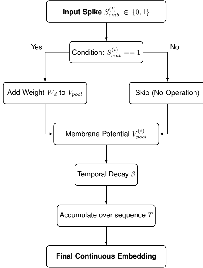
Figure 3: Internal computational flow of the purely recurrent Add-Only Pooler. Floating-point multiplications are completely eliminated.
