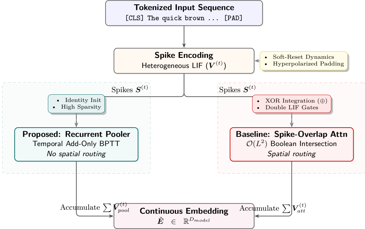
Figure 1: Architectural flowchart contrasting the proposed minimalist Recurrent Pooler against the \mathcal{O}(L^2) Spike-Overlap Attention baseline. The Recurrent Pooler completely bypasses quadratic spatial routing, natively translating discrete token spikes into a continuous temporal embedding state.
