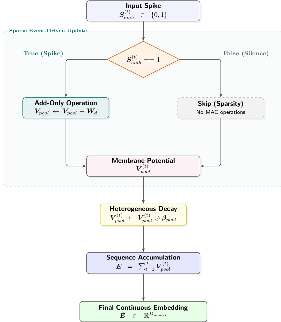
Figure 3: Internal computational flow of the purely recurrent Add-Only Pooler. Floating-point multiplications are completely eliminated.
