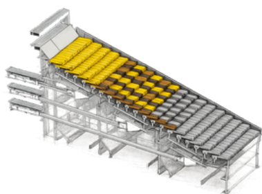
Combustion Grate Concept
