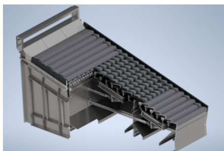
Combustion Grate Render
