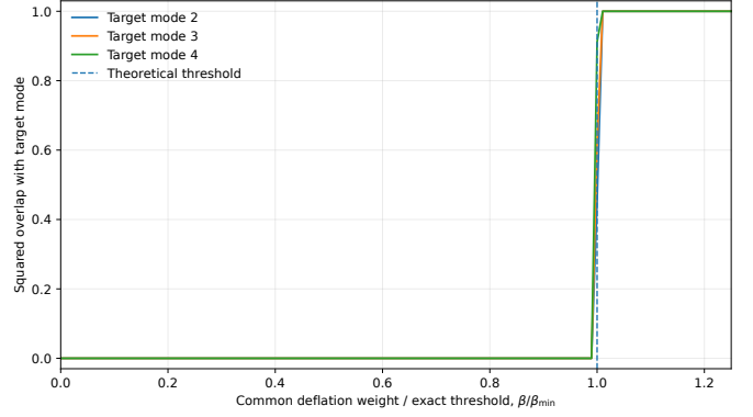
Fig. 2. Exact deflation sweep for target modes 2–4 on Benchmark C, computed from the exact padded spectrum with no sampling. The target becomes the ground state only after the penalty exceeds the spectral threshold in equation (22).
