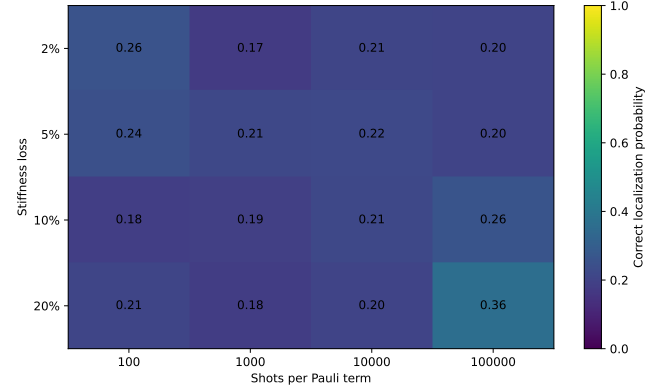
FIGURE 9. Correct damage-localization probability from independently sampled element-energy observables. The random-guess baseline is 1/6 = 16.7\% .
