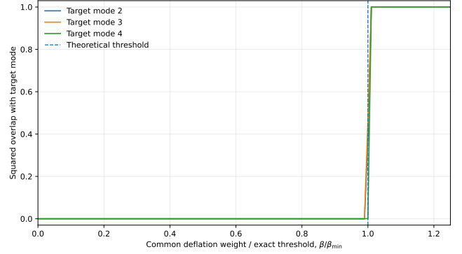
FIGURE 1. Exact deflation sweep for target modes 2–4. The target becomes the ground state only after the penalty exceeds the spectral threshold in equation (22).
