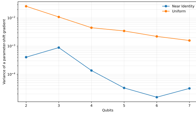
FIGURE 6. Empirical gradient variance for depth-2 real-amplitude circuits. The finite range is a diagnostic, not an asymptotic barren-plateau proof.
