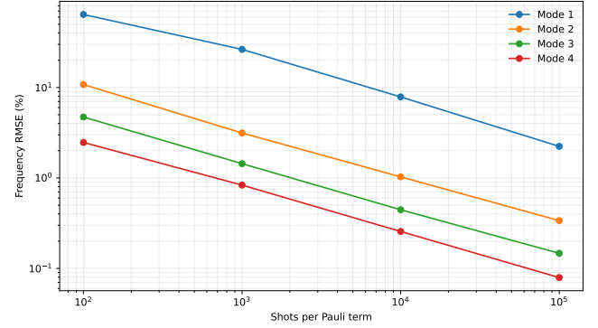
FIGURE 7. Finite-shot frequency RMSE from independent Pauli measurements of exact modal states.
