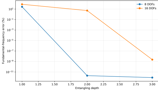
FIGURE 5. Fundamental-frequency error versus circuit depth for 8- and 16-DOF chain models.
