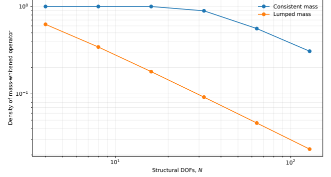
FIGURE 3. Density of the mass-whitened operator. Consistent mass introduces substantially more long-range coupling than lumped mass in the tested chains.
