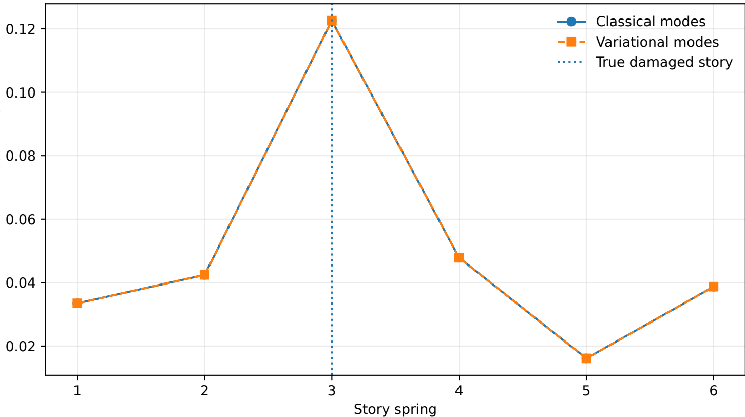
Four-mode strain-energy change index
