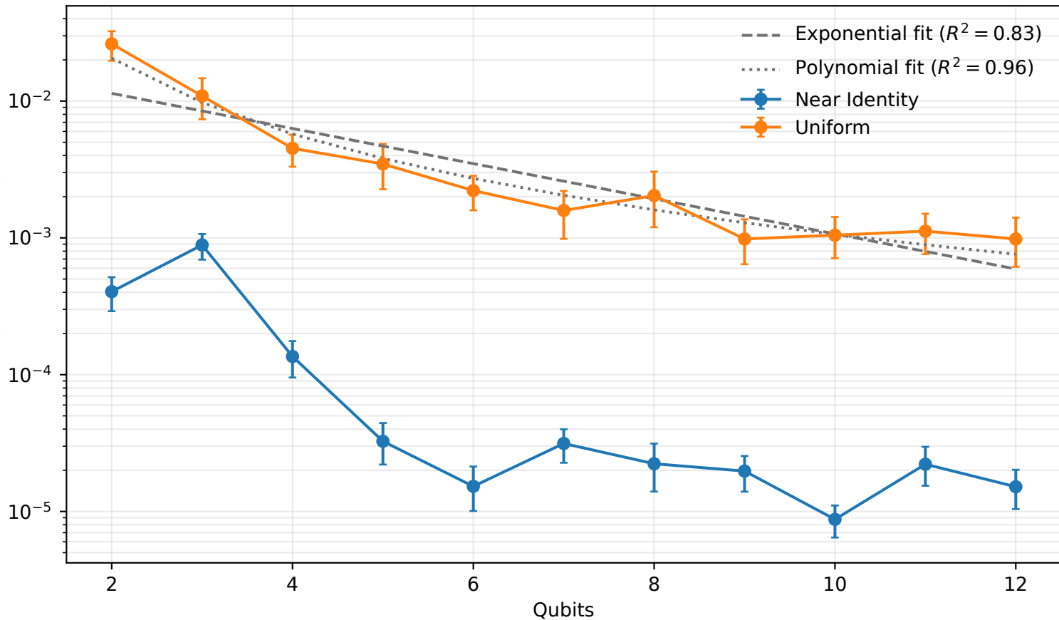
Variance of a parameter-shift gradient
