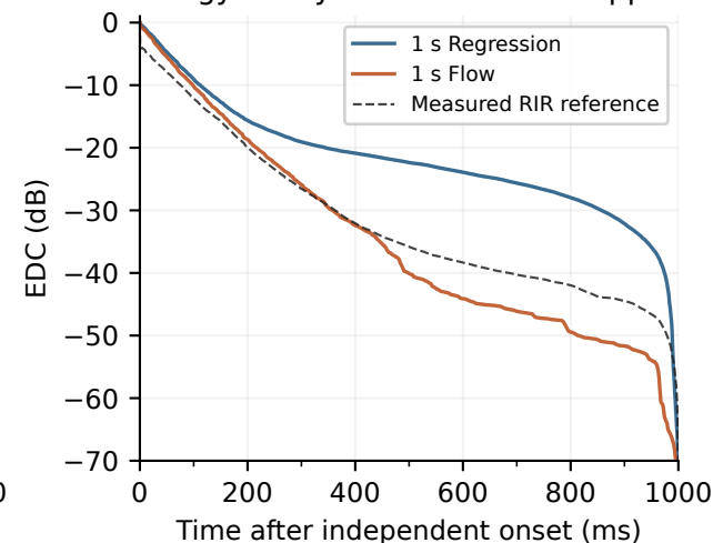
Energy decay over measured support
