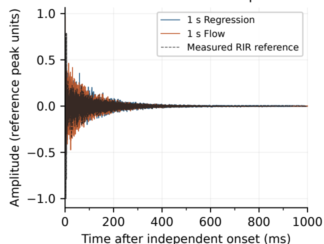
RIR: measured reference and predictions
