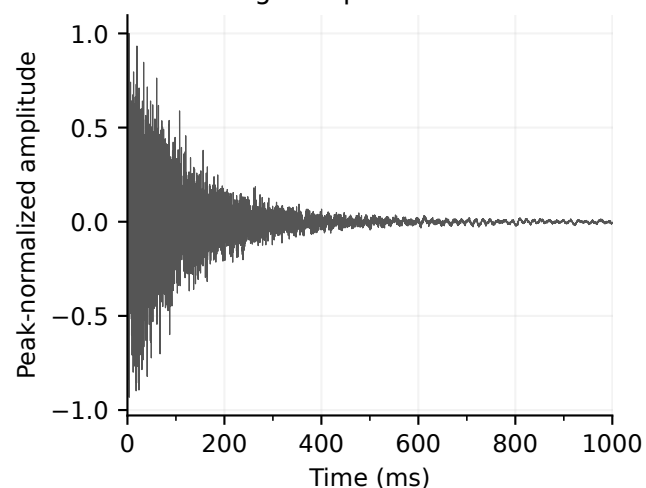
Room 4, position 6, EM32 Single-clap observation
