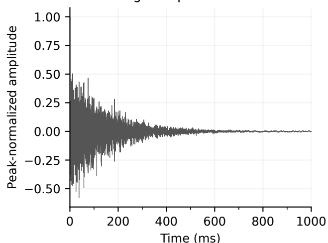
Room 6, position 4, EM64 Single-clap observation
