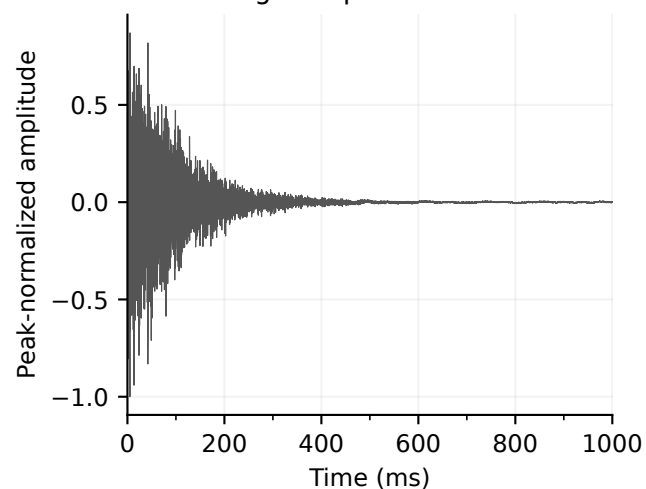
Room 6, position 4, EM64 Single-clap observation
