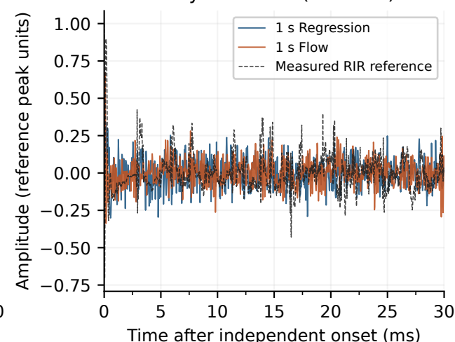
Early RIR detail (0-30 ms)
